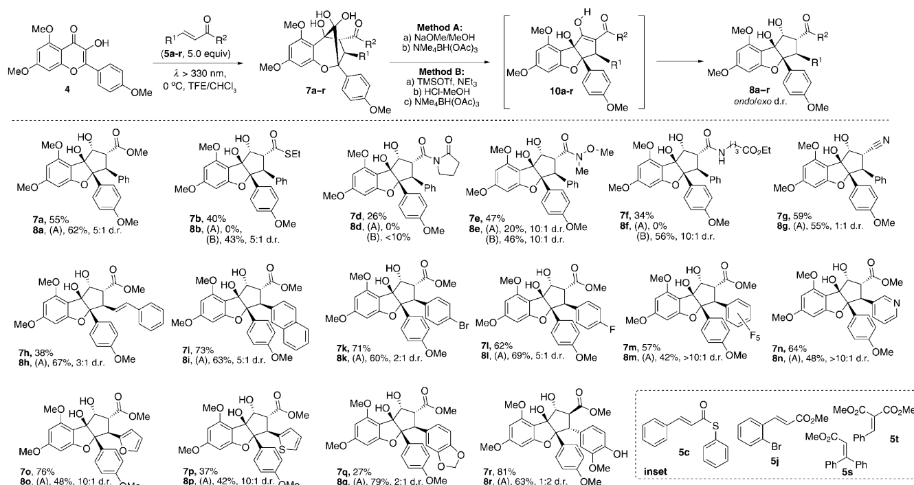
Scheme 2. Scope of the [3+2] photocycloaddition to produce aglains 7a-r and rocaglates 8a-r (major diastereomer shown, d.r. obtained by ^1\text{H} NMR). See the Supporting Information for details. TMS = trimethylsilyl, Tf = trifluoromethanesulfonyl.
