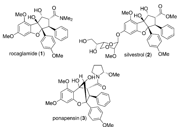
Figure 1. Representative aglain and rocaglate metabolites from Aglaia .
