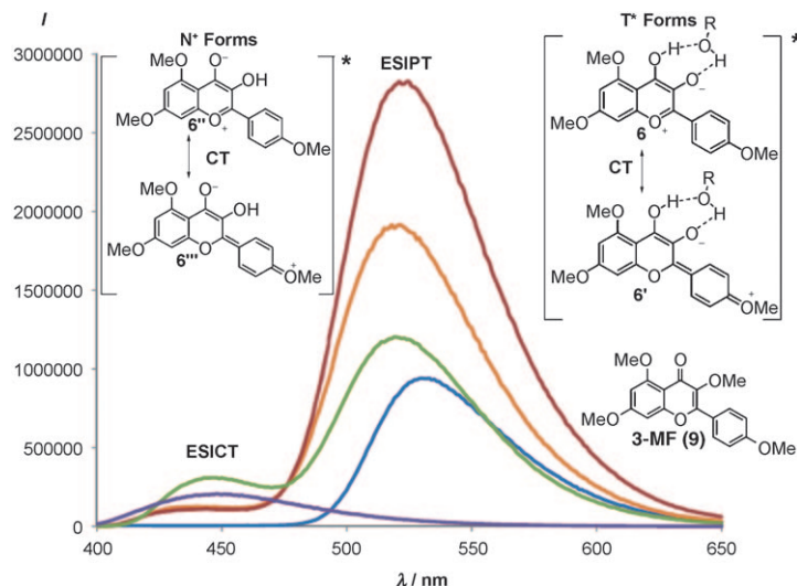
Figure 2. Fluorescence emission of 3-HF ( 4 ) and 3-MF ( 9 ) indicating both ESIPT and ESICT processes with presumed charge transfer (CT) in both excited states from phototautomers 6/6' and 6''/6''' . Light blue: 4 in \text{CHCl}_3 , orange: 4 in \text{CHCl}_3/\text{TFE} (95:05), red: 4 in \text{CHCl}_3/\text{TFE} (70:30), green: 4 in TFE, purple: 9 in TFE.
